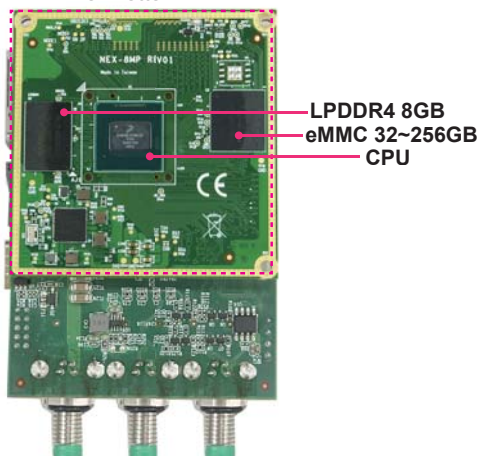
NXP-HAI02-Bottom
