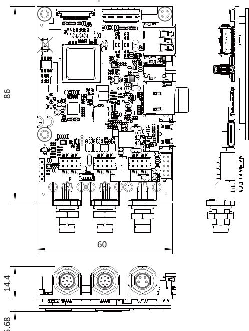
NXP-HAI02-Top
